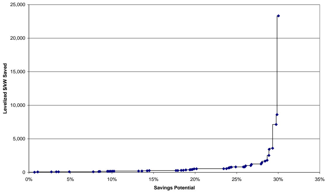
Supply Curve - Capacity (S_Aereui.Xls) 52 Measures
