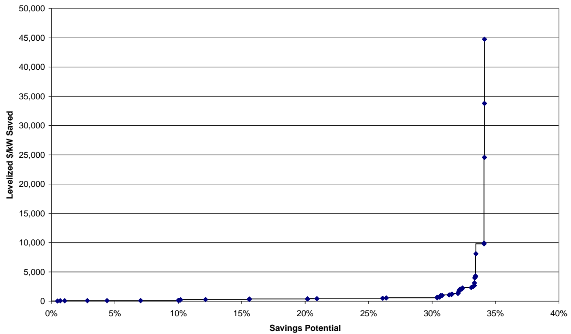
Supply Curve - Capacity (S_Aernclp.Xls) 47 Measures
