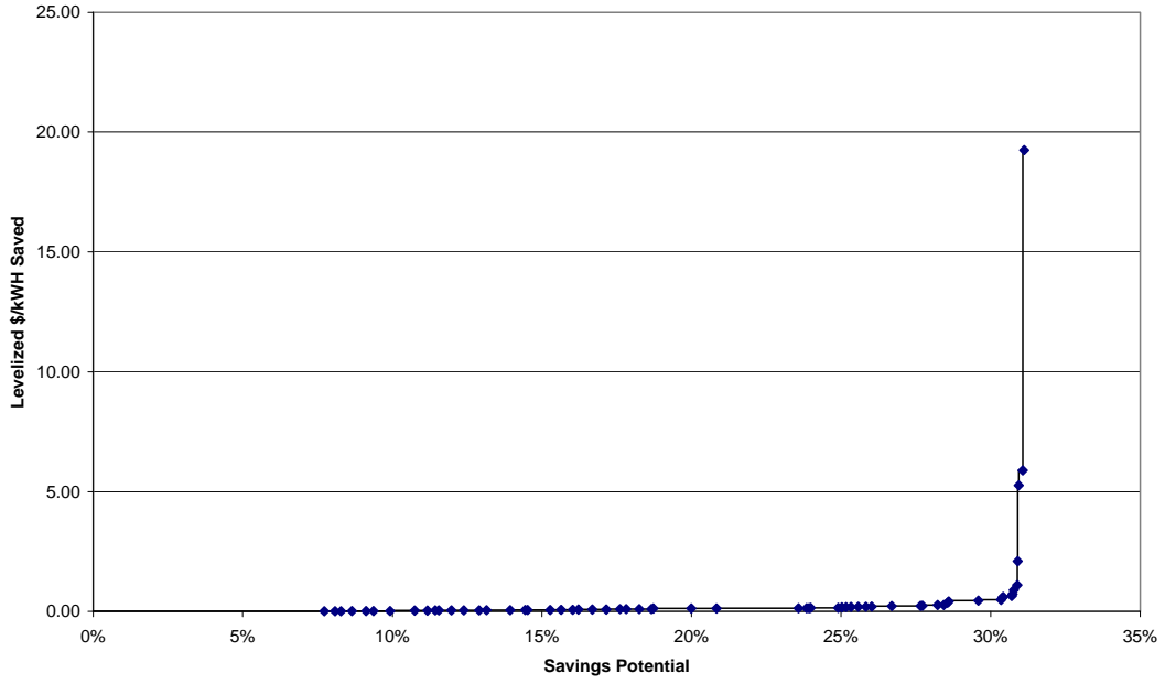
Supply Curve - Energy (S_Aereui.Xls) 61 Measures
